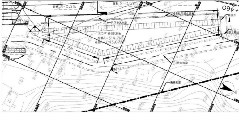
Plan view of SDP1
