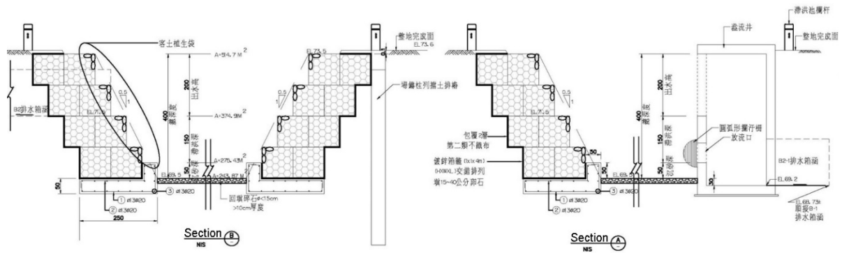
Figure 7 The plan and sections views of SDP1
