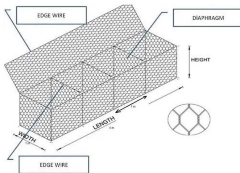
Figure 5 The regular assembly of the wire mesh cages [11]
