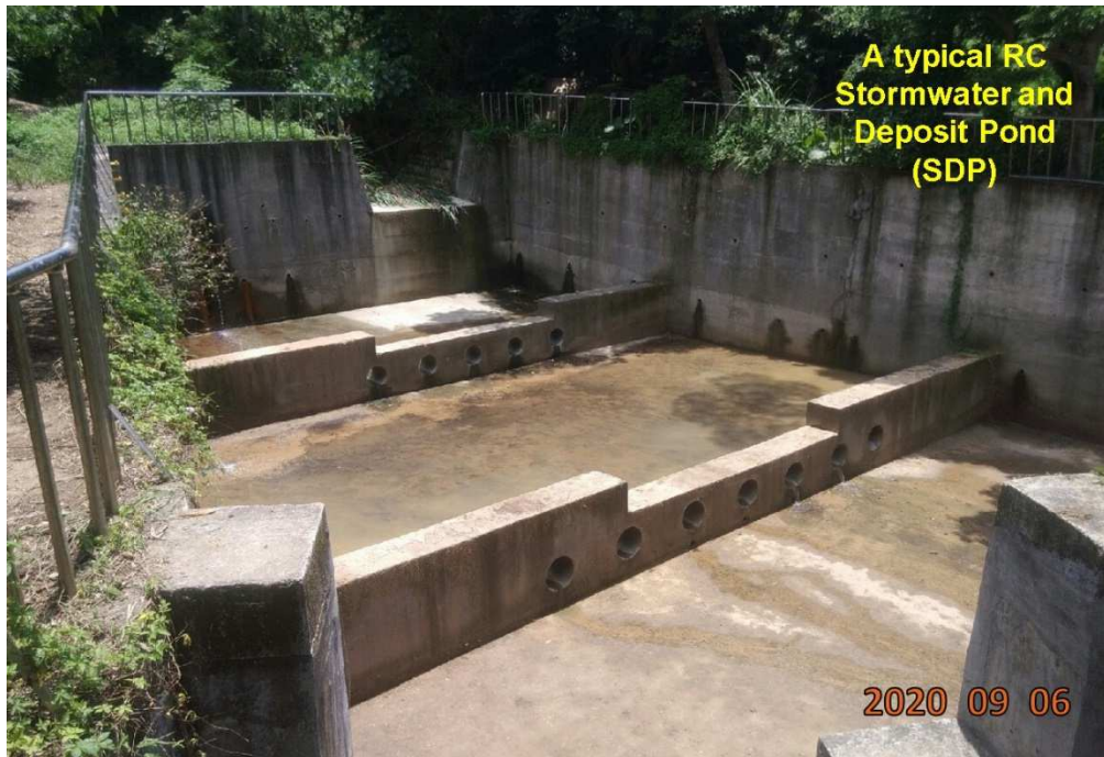
Figure 4 The photo of a typical RC SDP
