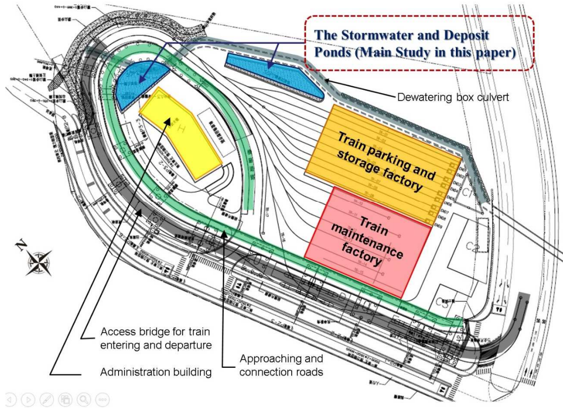
Figure 1 The layout for the depot zone of the ALRMS project
