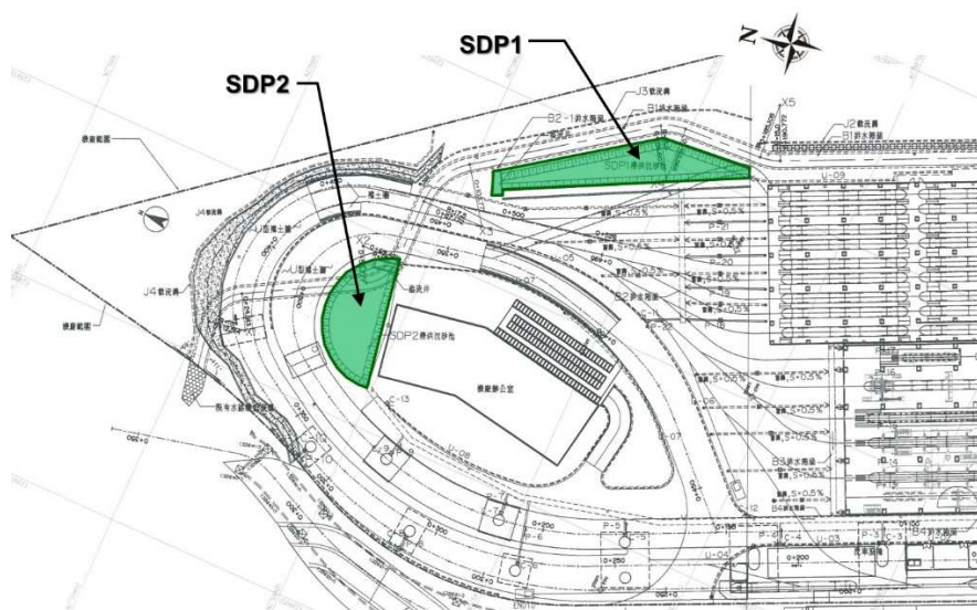
Figure 3 The location of two SDPs in the depot zone of the ALRMS project
